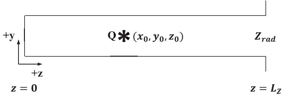
Figure 2-1 – Schematic of the idealized model setup. A point source is placed in a finite duct of length L_z at the location (x_0, y_0, z_0) . The sides of the duct and the boundary at z = 0 are assumed rigid, but the end of the duct ( z = L_z ) has a finite, non-zero radiation impedance boundary condition Z_{rad} .
